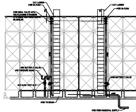
IN-FLOW ELEVATION SCALE 1/50
