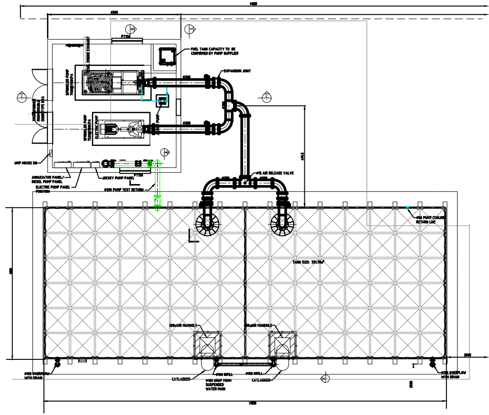
PUMP HOUSE LAYOUT SCALE 1/50
