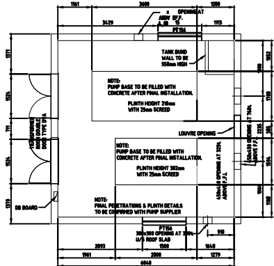
BUILDERS WORK SCALE 1/50
