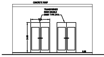
FRONT WALL ELEVATION SCALE 1/50
