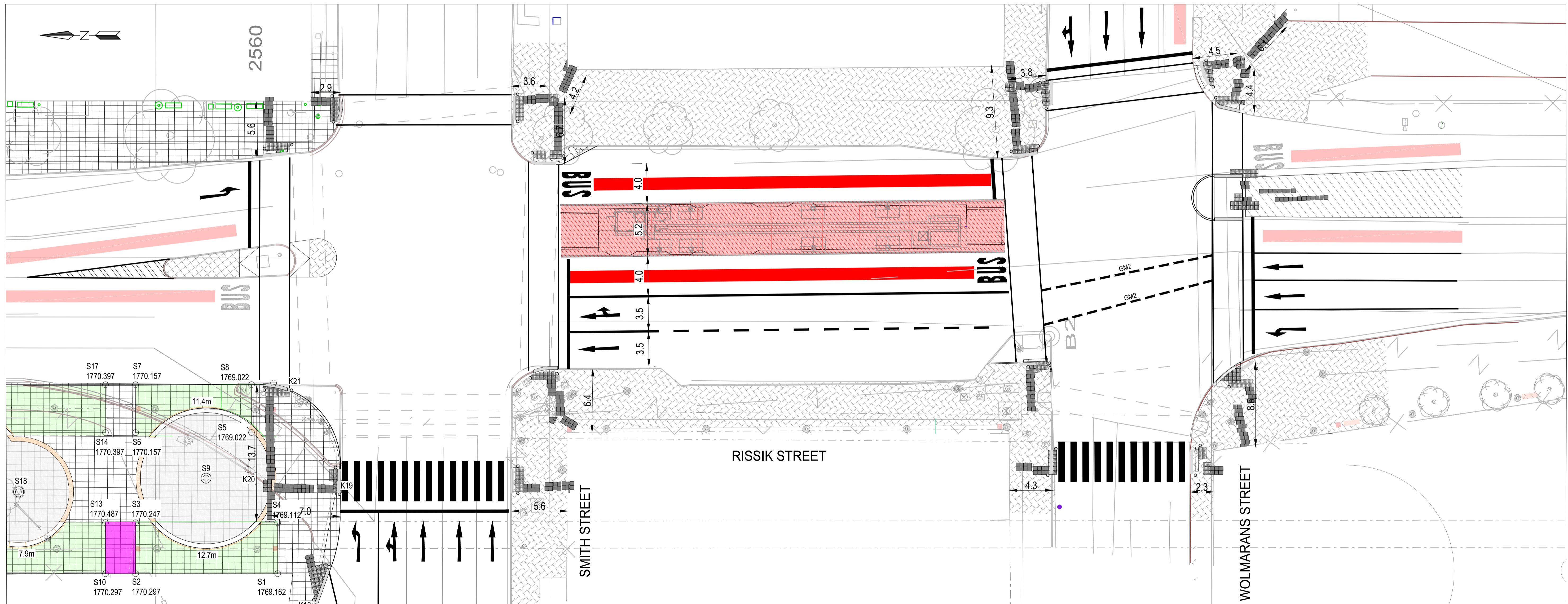
RISSIK STREET BRT LAYOUT PLAN SCALE = 1:500
